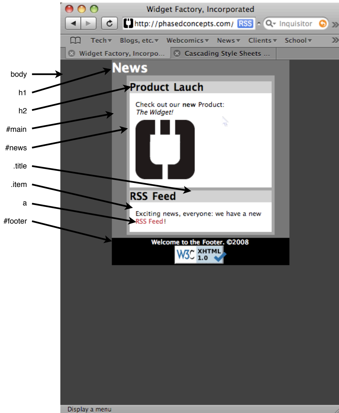
Figure 4.1: Example 2 Rendered w/CSS File (Example 3)
